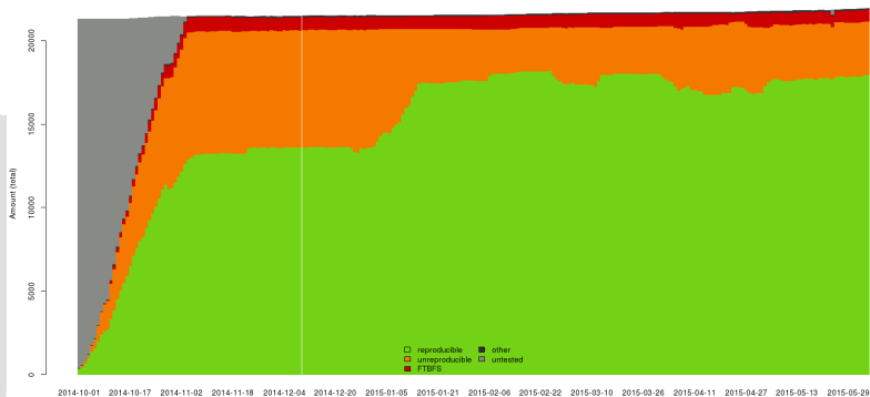
Reproducibility status for packages in 'unstable'
